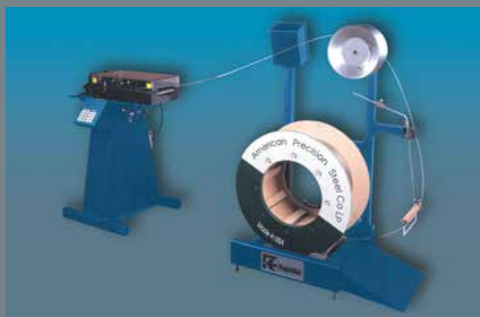
Complete cut-to-length line: SCL125S + CB16A + W6S air feed CTL machine and RD317S rim drive payout reel (loop is developed behind and above reel to save space).
